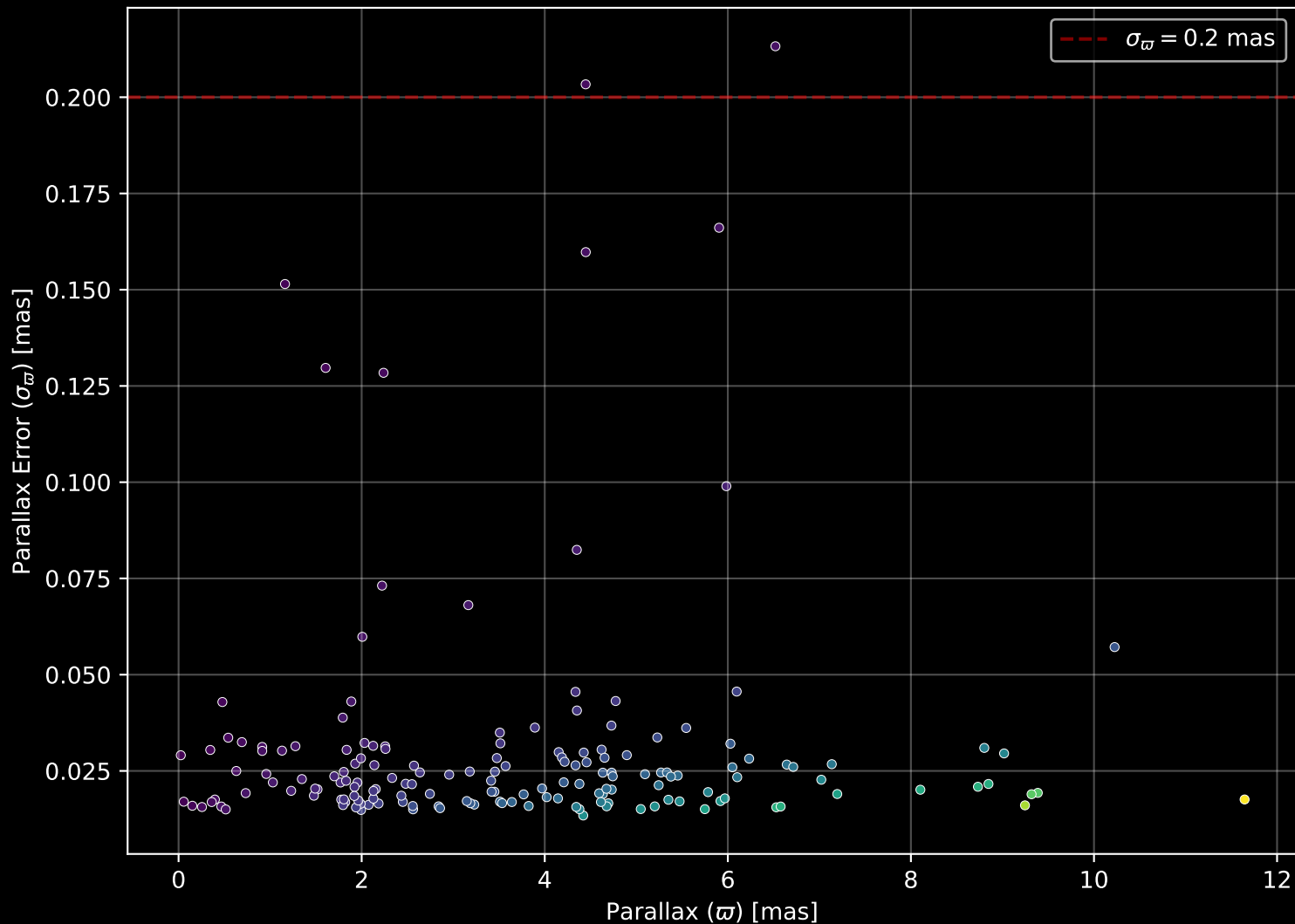
APOGEE DR17 Field: [049+88_MGA] Parallax Quality (n= 167)
