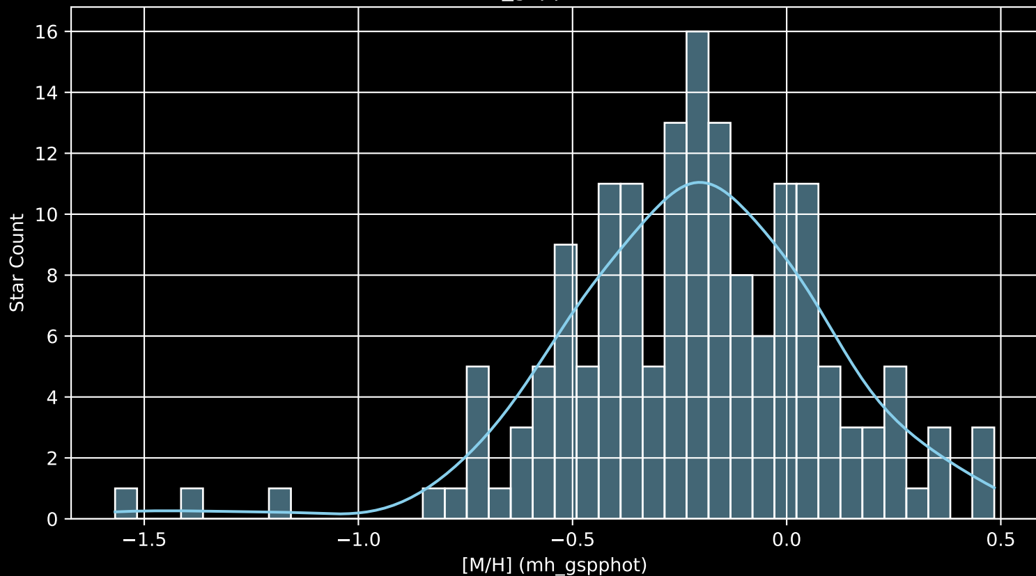
APOGEE DR17 Field: [049+88_MGA [M/H] (mh_gspphot) (n= 161)
