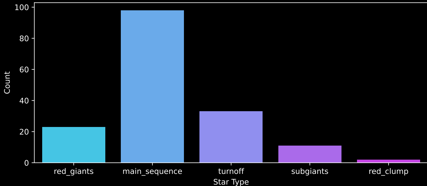
APOGEE DR17 Field: [049+88_MGA] Count plot of Star Type
