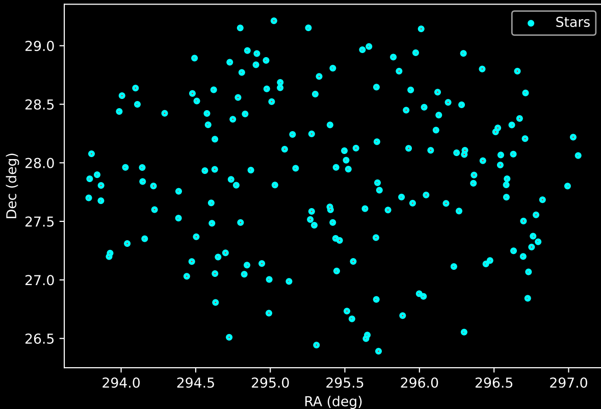
APOGEE DR17 Field: [049+88_MGA] Proper Motion Vectors for Gaia Star Field (n= 167)
