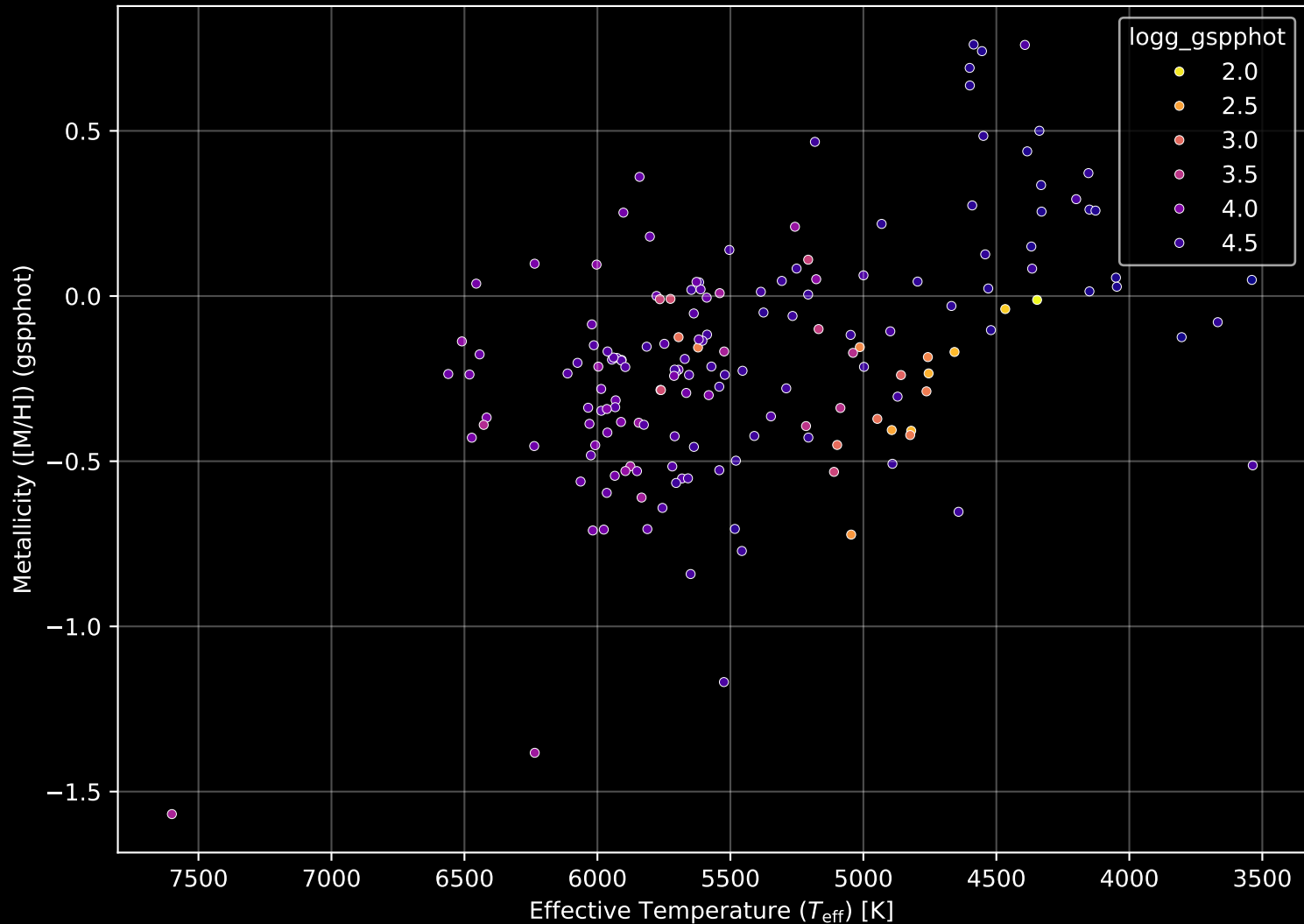
APOGEE DR17 Field: [049+88_MGA] Stellar Population Parameters (n= 167)
