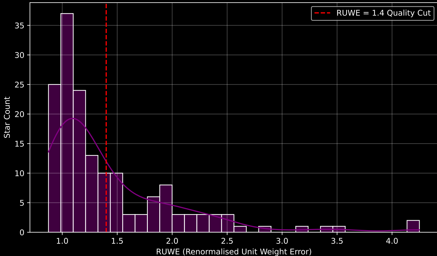
GAPOGEE DR17 Field [049+88_MGA] RUWE Distribution (n= 161)
