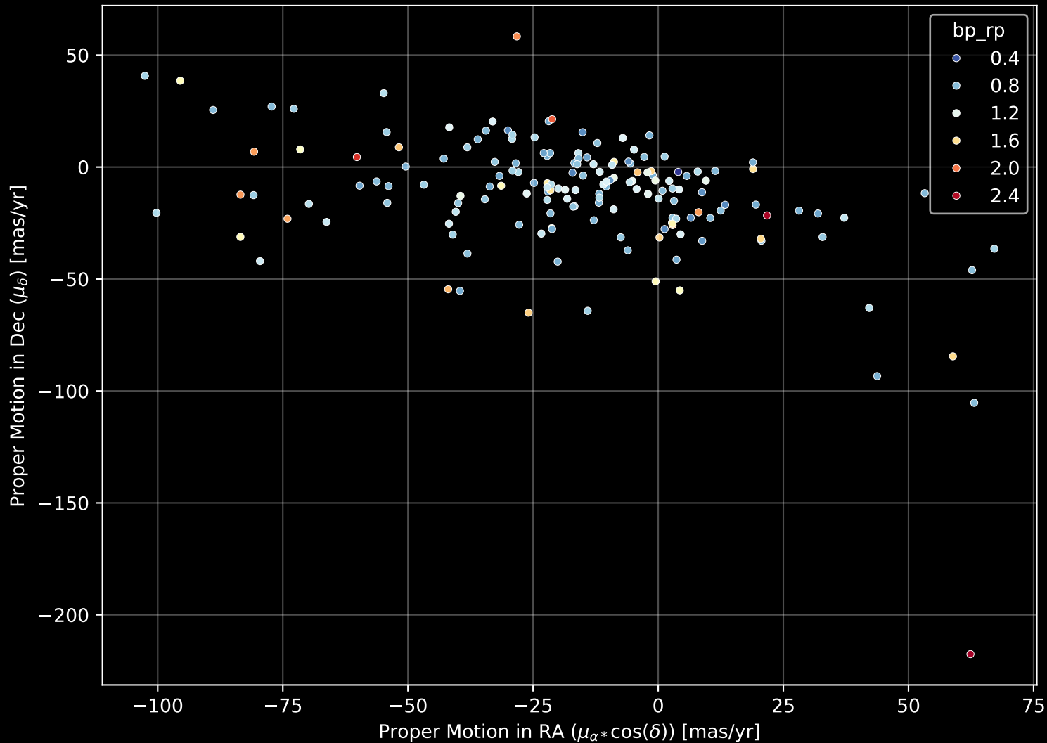
APOGEE DR17 Field: [049+88_MGA] Proper Motion Diagram (n= 167)
